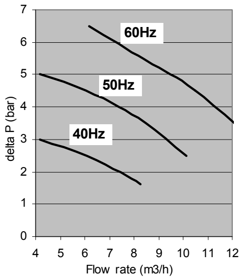
Hydraulic Performance
