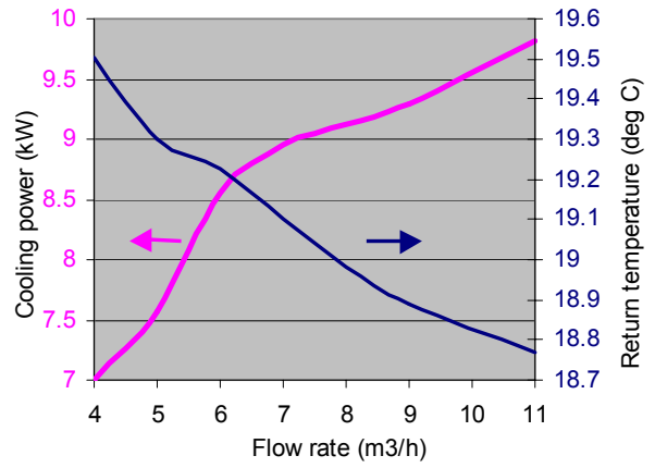
Thermal performance with fridge ON for a fixed supply temperature=18°C
